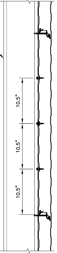
(FP4) SIDE JOINT AND (3) FAB-LOKS
