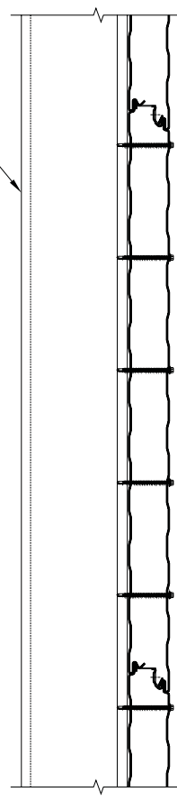
(FP9) (4) SELF-DRILLING OR SELF-TAPPING FASTENERS W/ NEOPRENE BONDED WASHER
