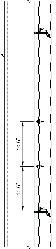
(FP3) SIDE JOINT AND (2) FAB-LOKS
