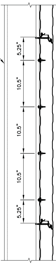
(FP5) SIDE JOINT AND (4) FAB-LOKS
