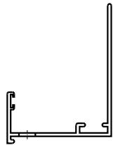
2" BASE EXTRUSION [9405A]
