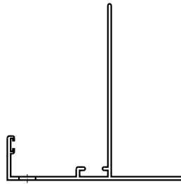
2" BASE/SOFFIT EXTRUSION [9414A]
