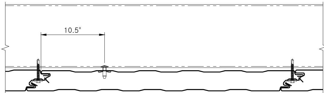
FASTENING PATTERN 2 SIDE JOINT FASTENING AND ONE DOME HEAD BULB-TITE® RIVET
