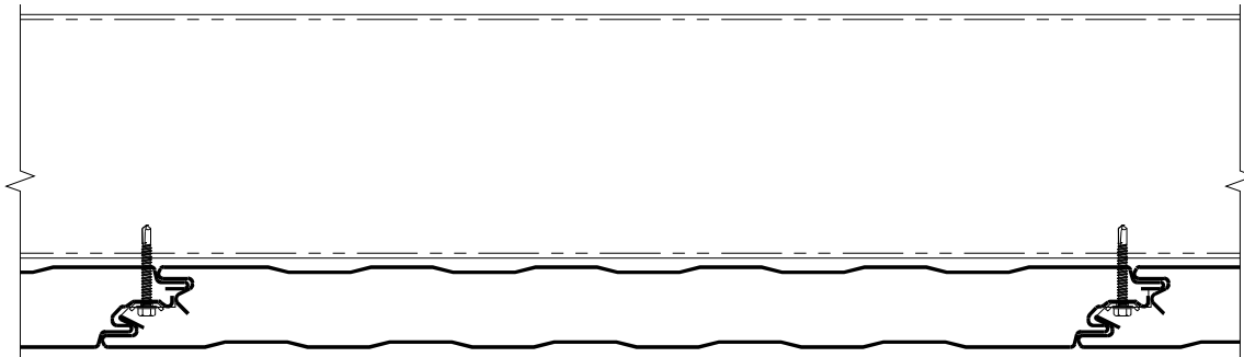
FASTENING PATTERN 1 SIDE JOINT FASTENING
