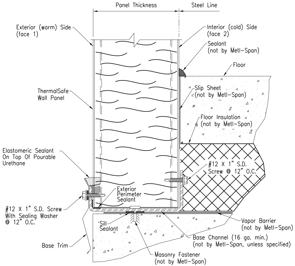
Vertical Panel-Base Detail (Base Channel)
