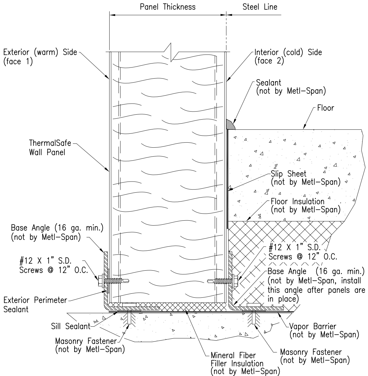
Vertical Panel-Base Detail (Isolated Base Angles)
