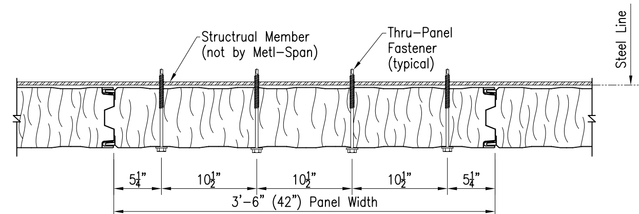
FASTENER PATTERN 2
