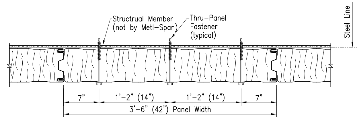
FASTENER PATTERN 1
