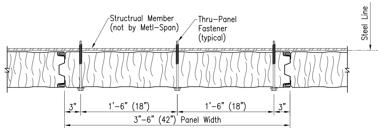
FASTENER PATTERN 1
