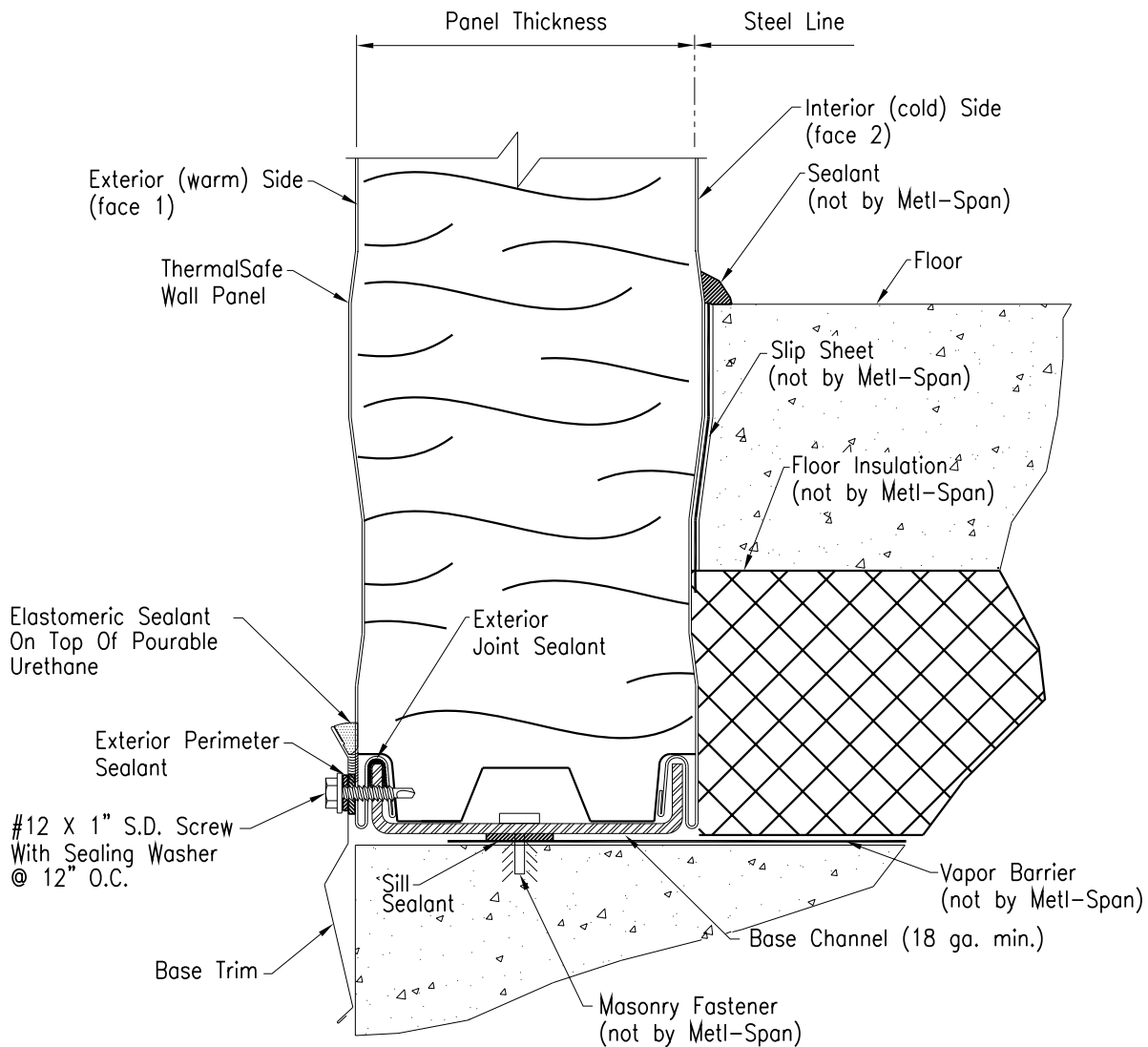
Horizontal Panel-Base Detail
