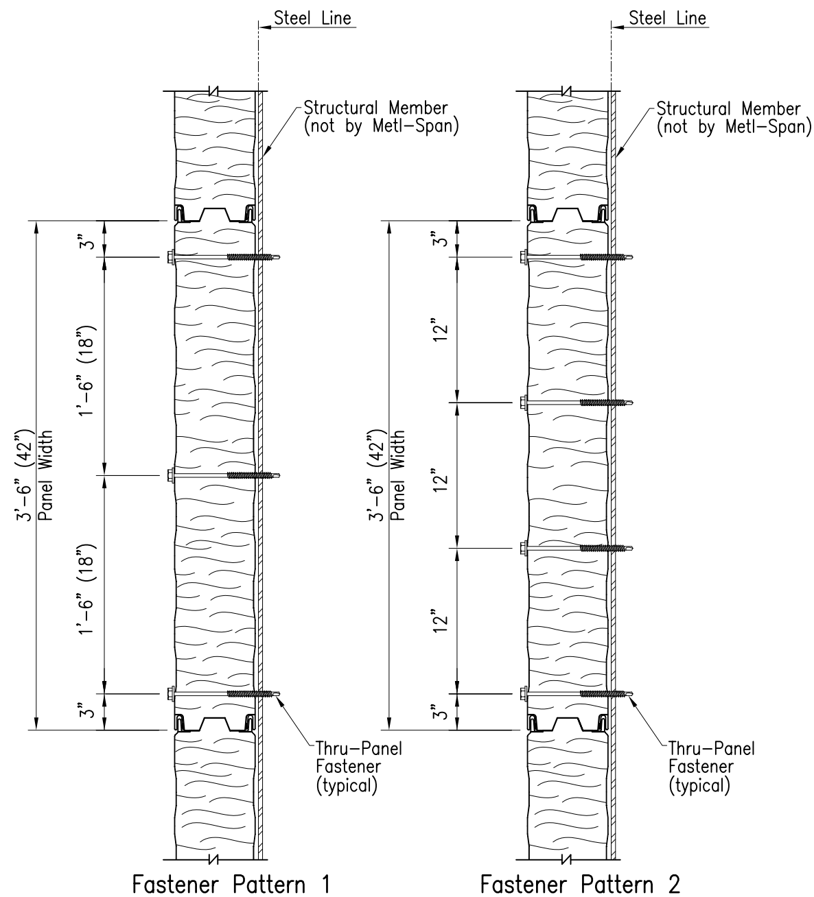
Horizontal Panel-Thru-Panel Fastener Patterns (@ Vertical Joint And Corner Structural)
