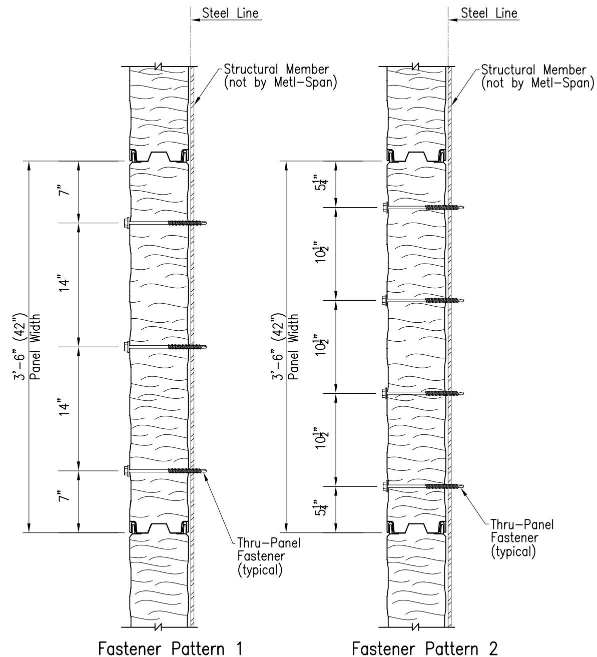
Horizontal Panel-Thru-Panel Fastener Patterns (@ Intermediate Structural)
