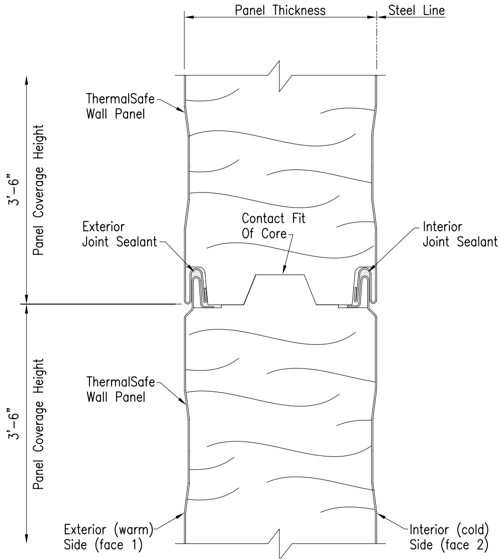
Horizontal Panel-Joint Detail
