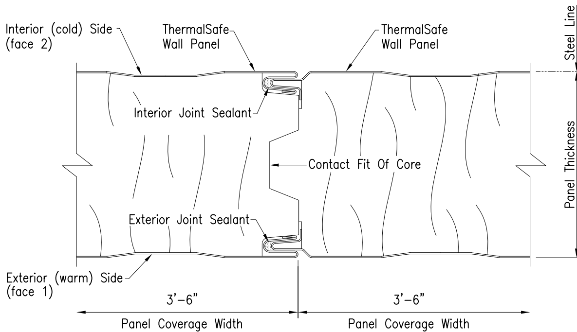
Vertical Panel-Joint Detail (Plan View)
