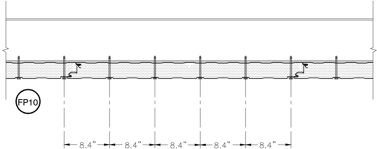
FASTENING PATTERN 10 WITH FIVE SELF-TAPPING SCREWS WITH MIN. 20 GA. NEOPRENE BONDED WASHER.
