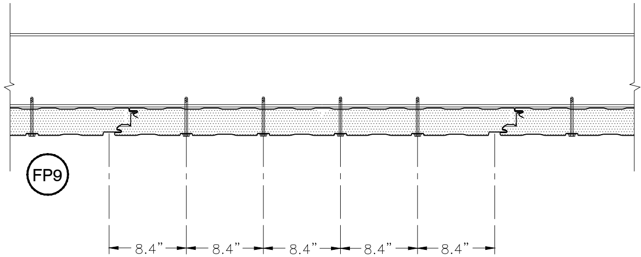
FASTENING PATTERN 9 WITH FOUR SELF-TAPPING SCREWS WITH MIN. 20 GA. NEOPRENE BONDED WASHER.
