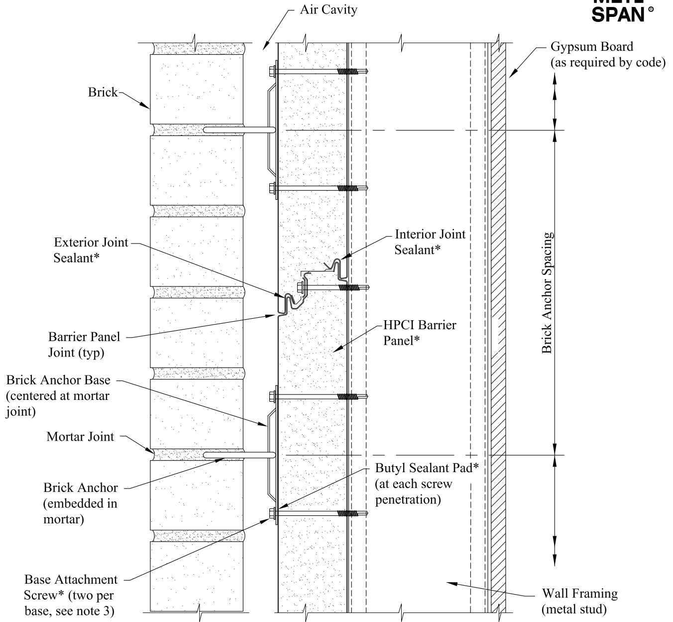
General Wall Section
