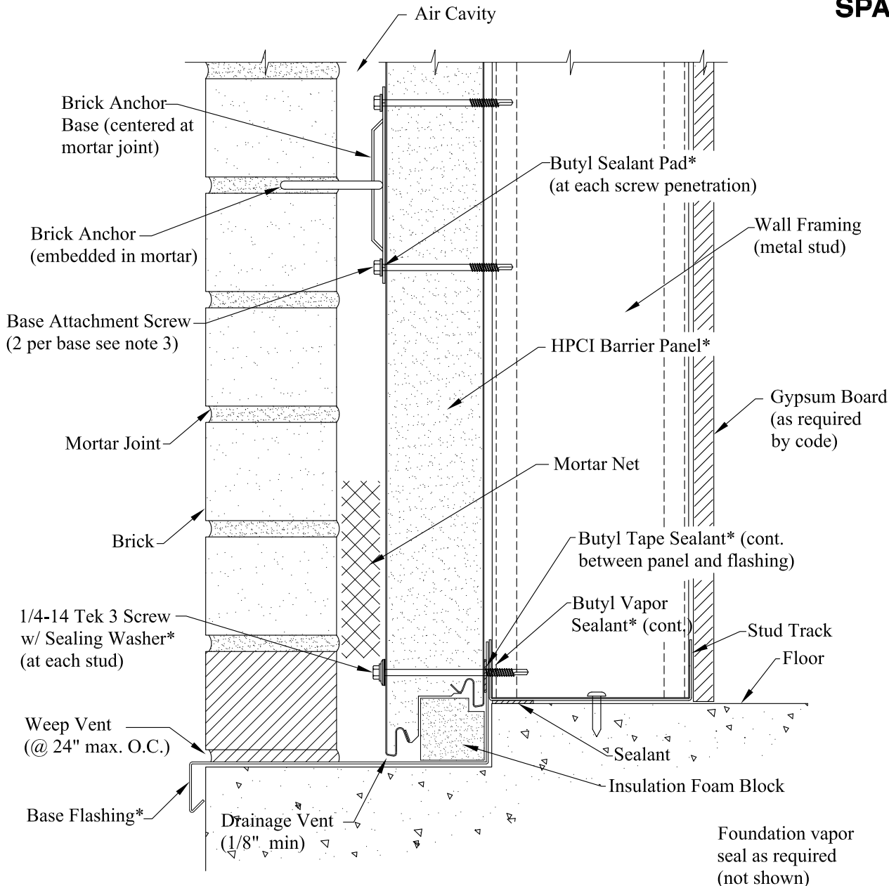
Wall Section @ Base (Foundation Ledge w/ Metal Flashing)
