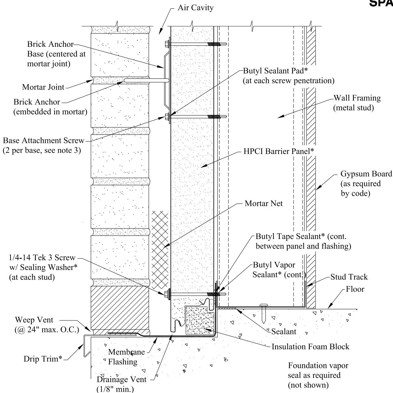
Wall Section @ Base (Foundation Ledge w/ Membrane Flashing)
