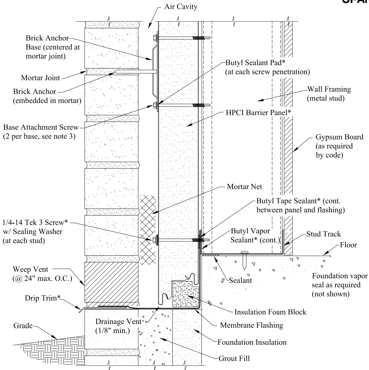
Wall Section @ Base (Brick Below Grade)
