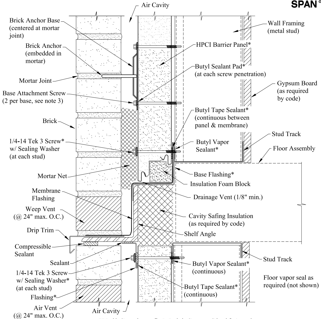
Wall Section @ Multi-Story Shelf Angle
