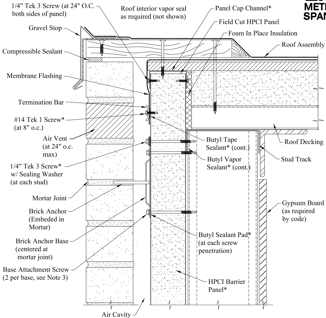
Wall Section @ Eave
