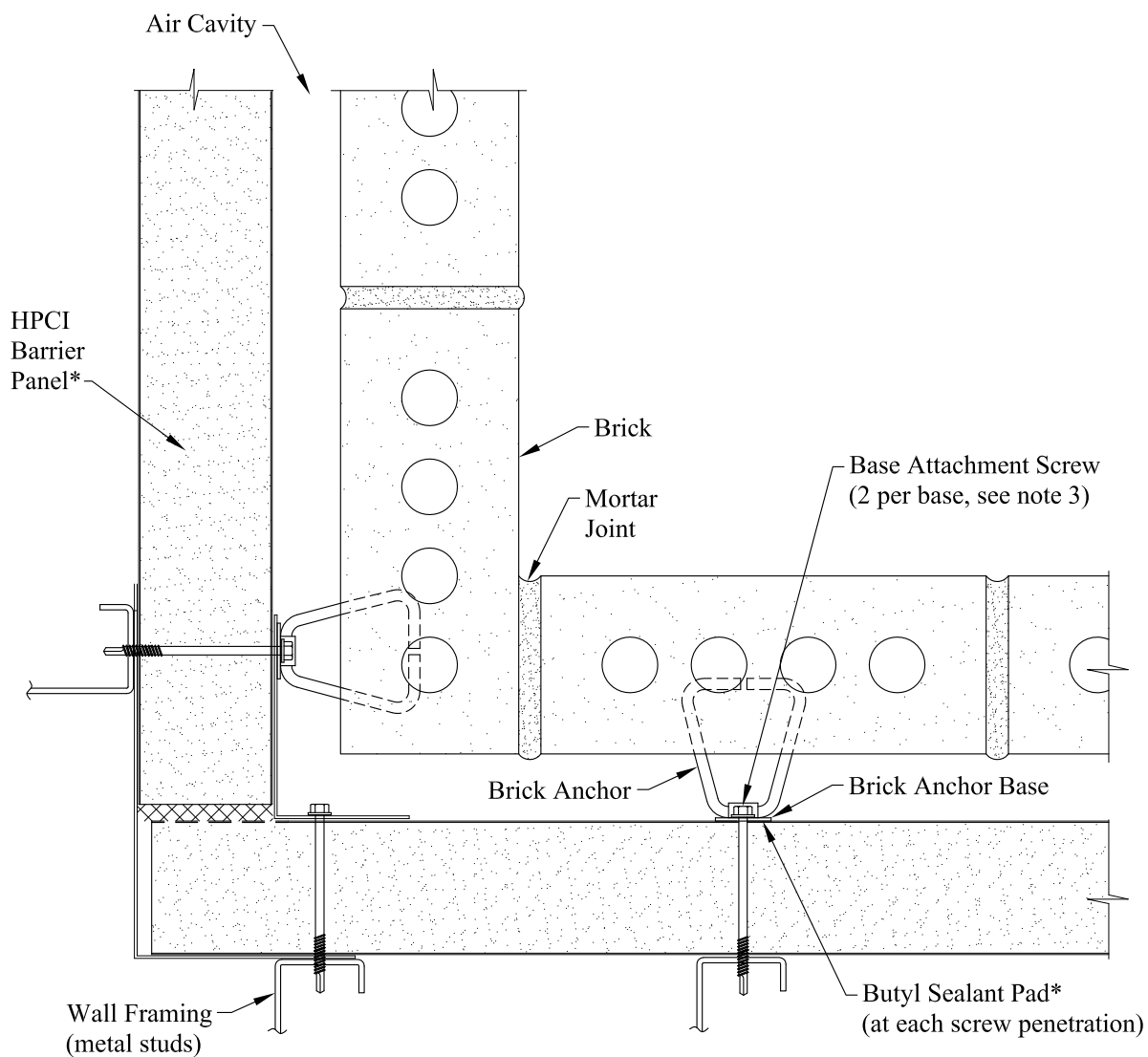
Wall Plan @ Inside Corner
