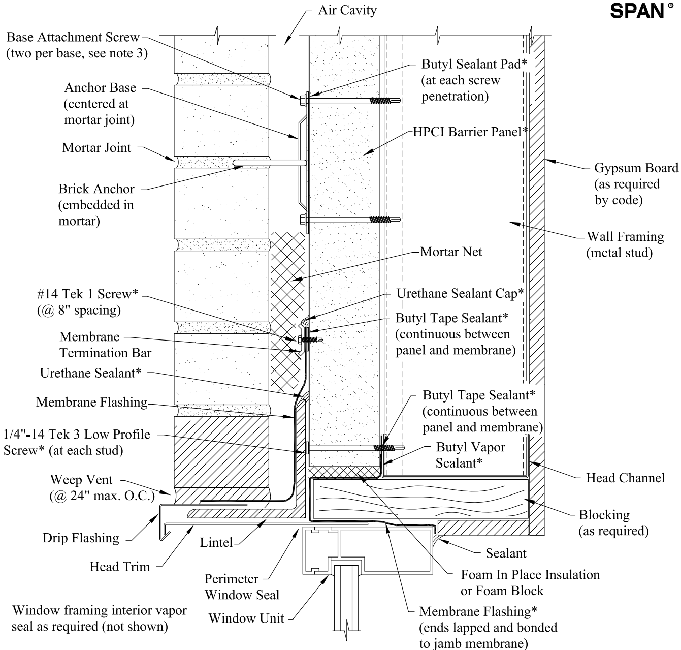
Wall Section At Window Head
