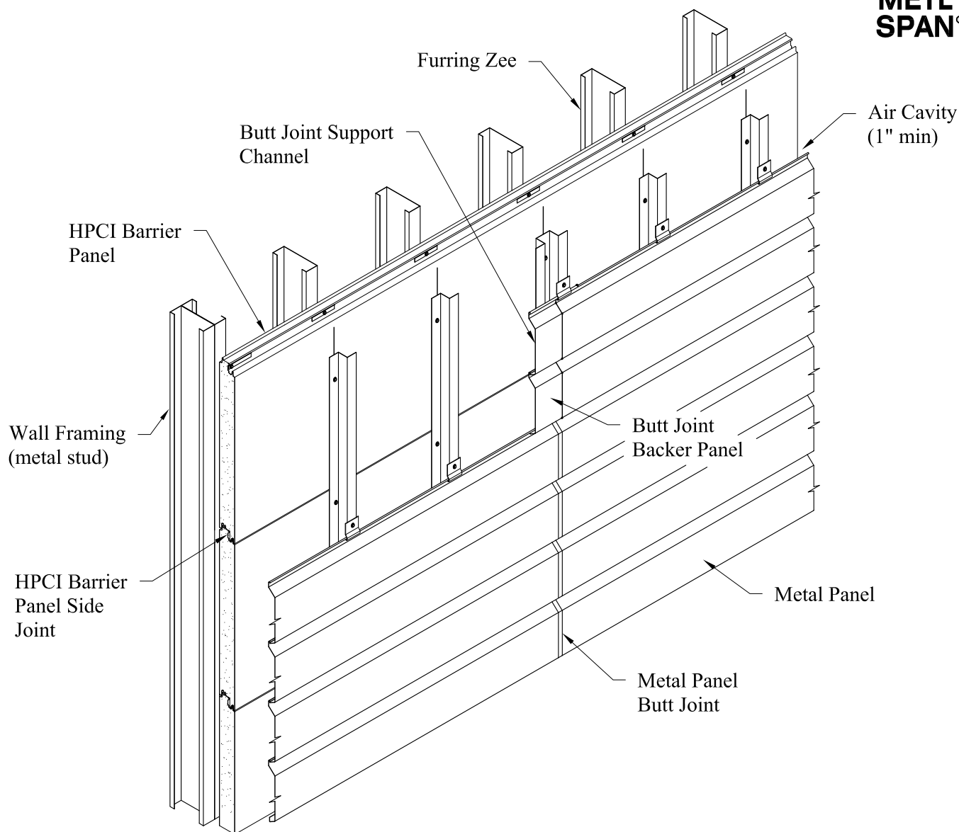
General Wall Assembly
