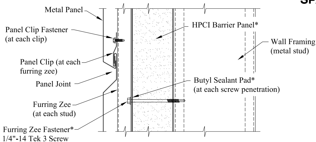
Assembly Section
