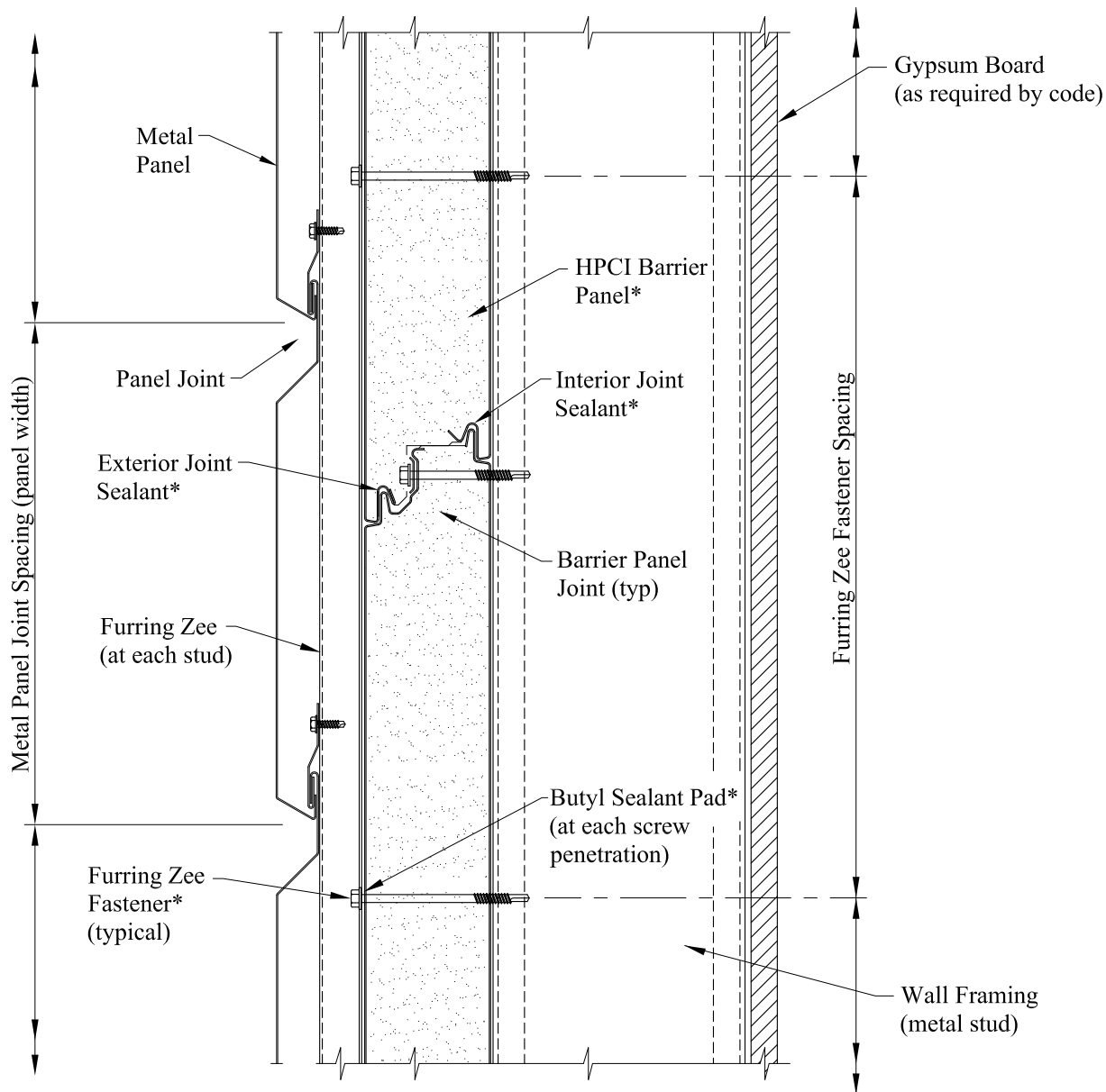
General Wall Section
