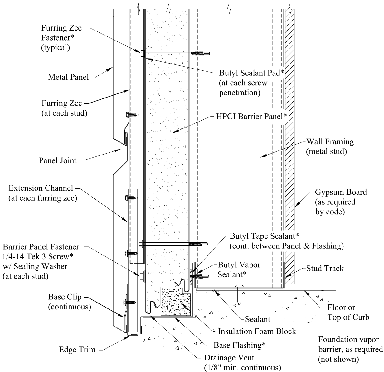
Wall Section @ Base
