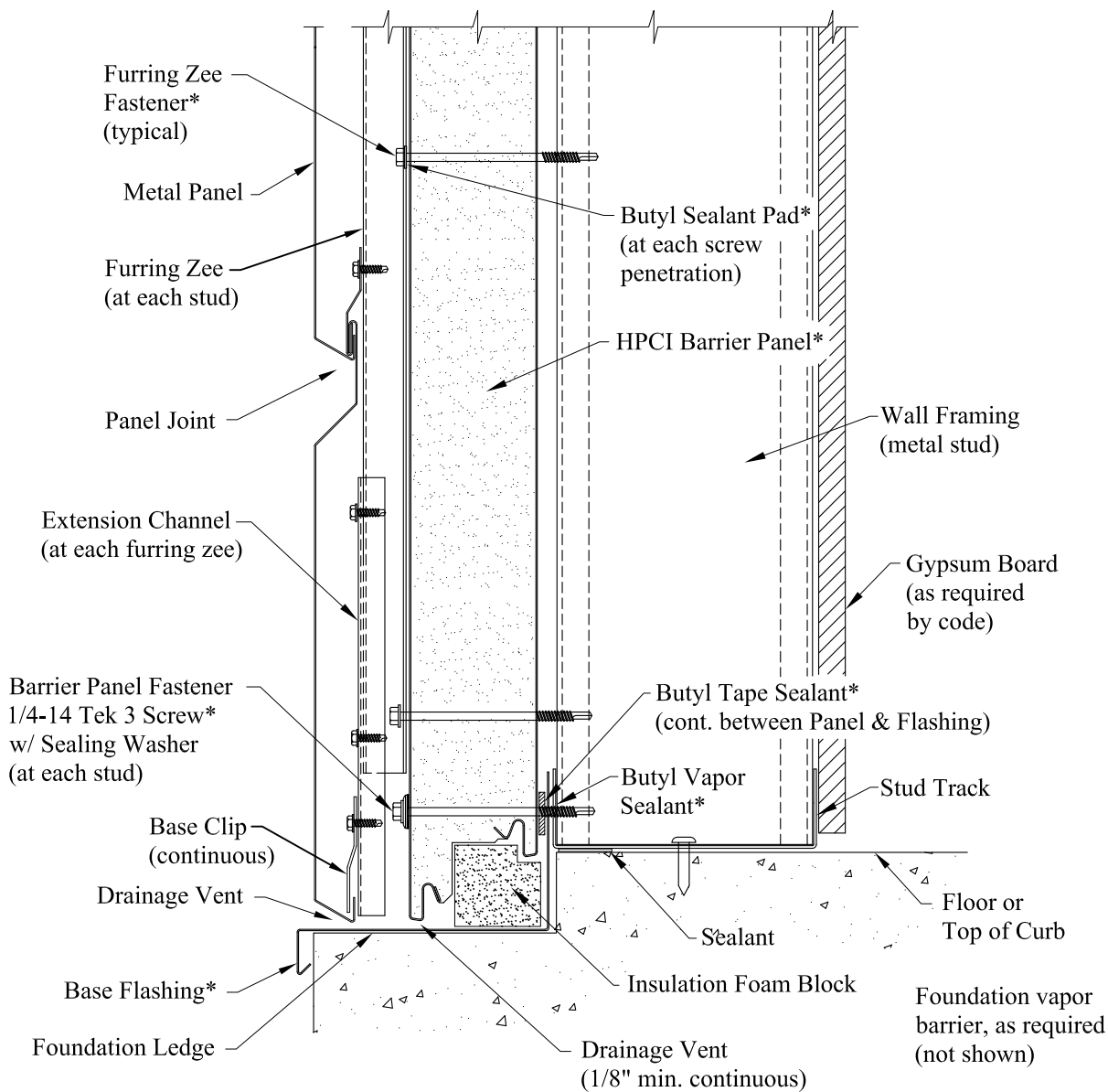
Wall Section @ Base (Extended Foundation Ledge)
