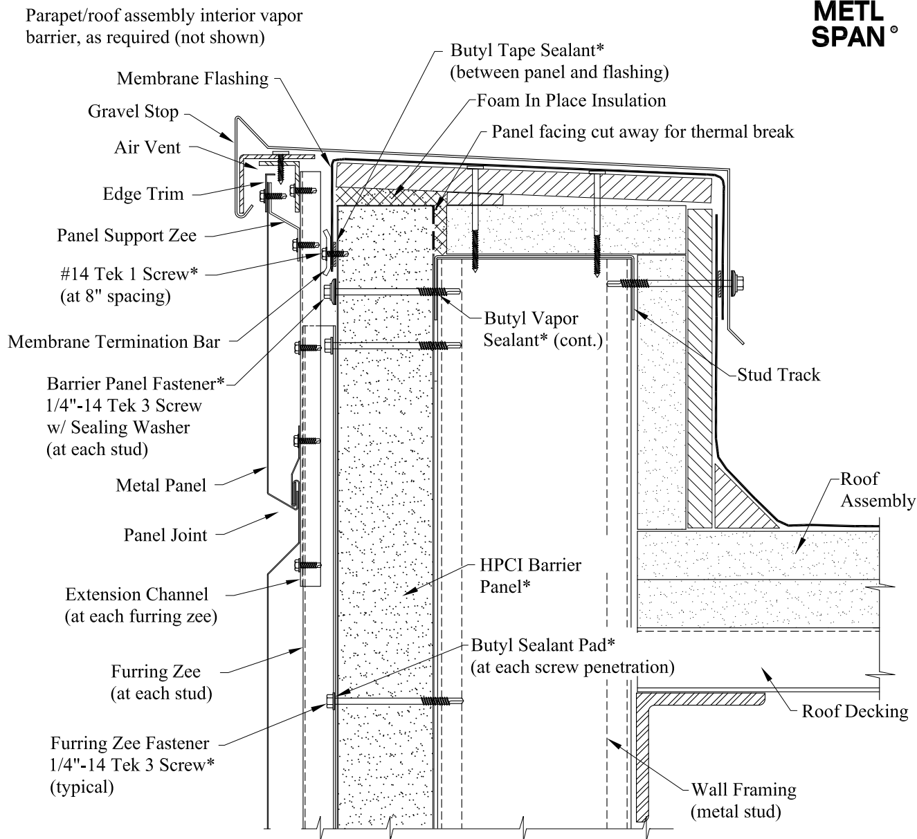
Wall Section At Parapet
