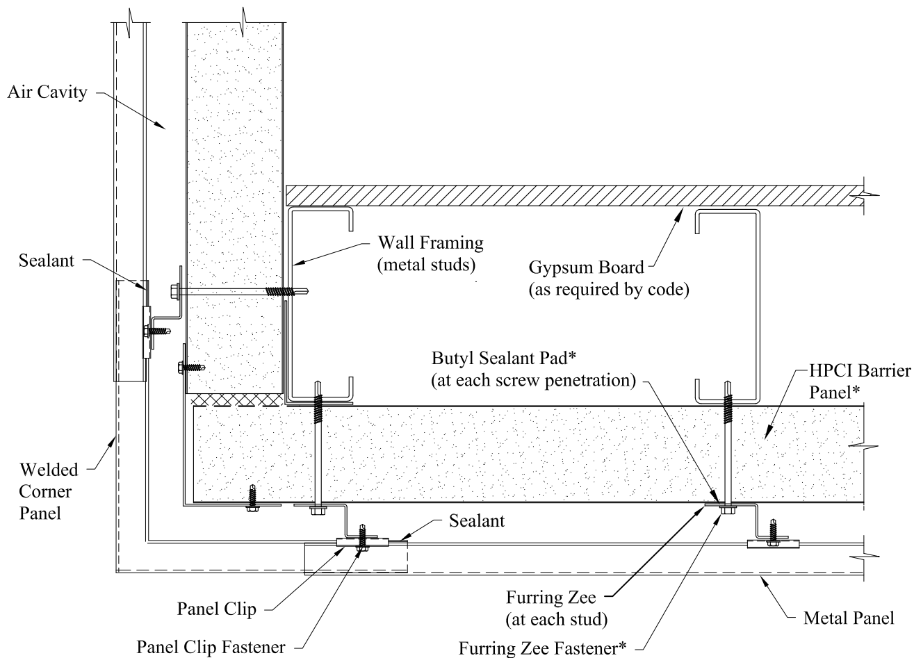
Wall Plan @ Outside Corner
