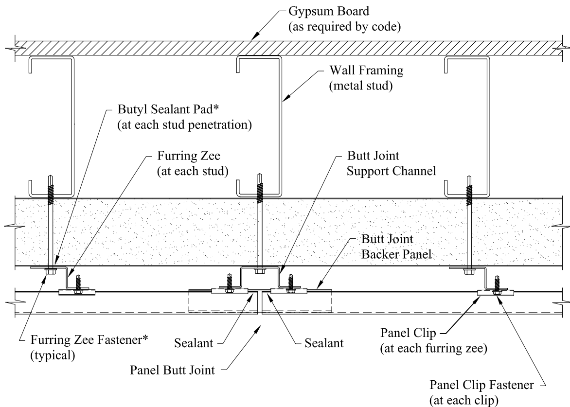
Wall Plan @ Panel Butt Joint
