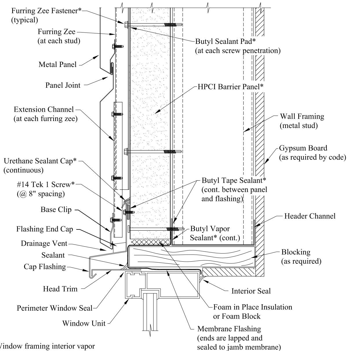
Wall Section @ Window Head
