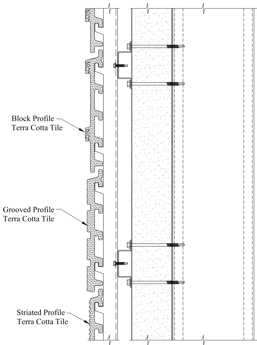
Wall Section with Typical Tile Options
