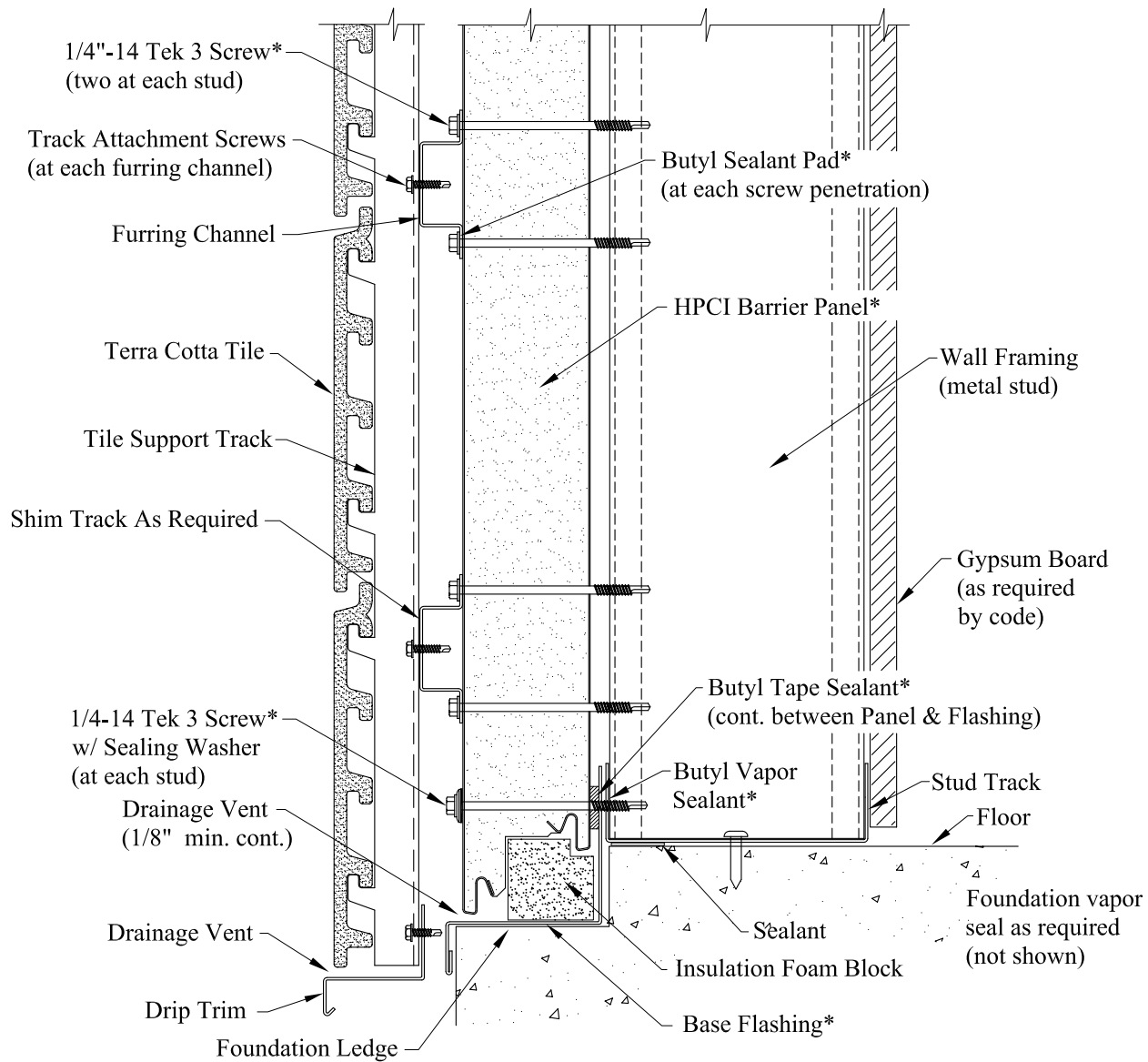
Wall Section @ Base (Recessed Ledge)
