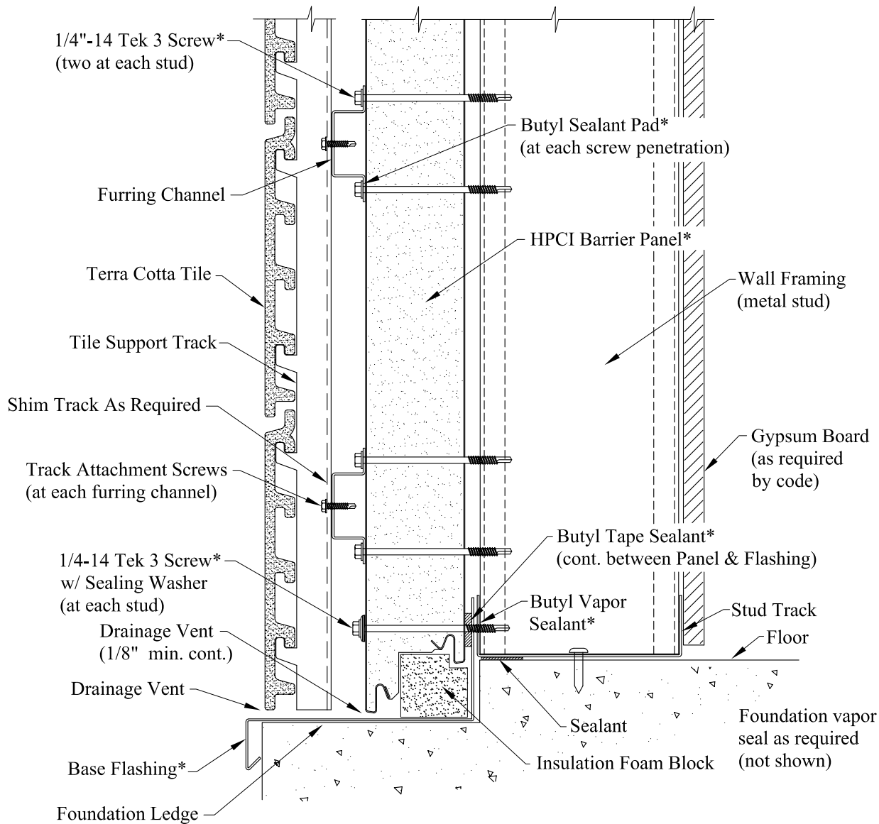
Wall Section @ Base (Extended Ledge)
