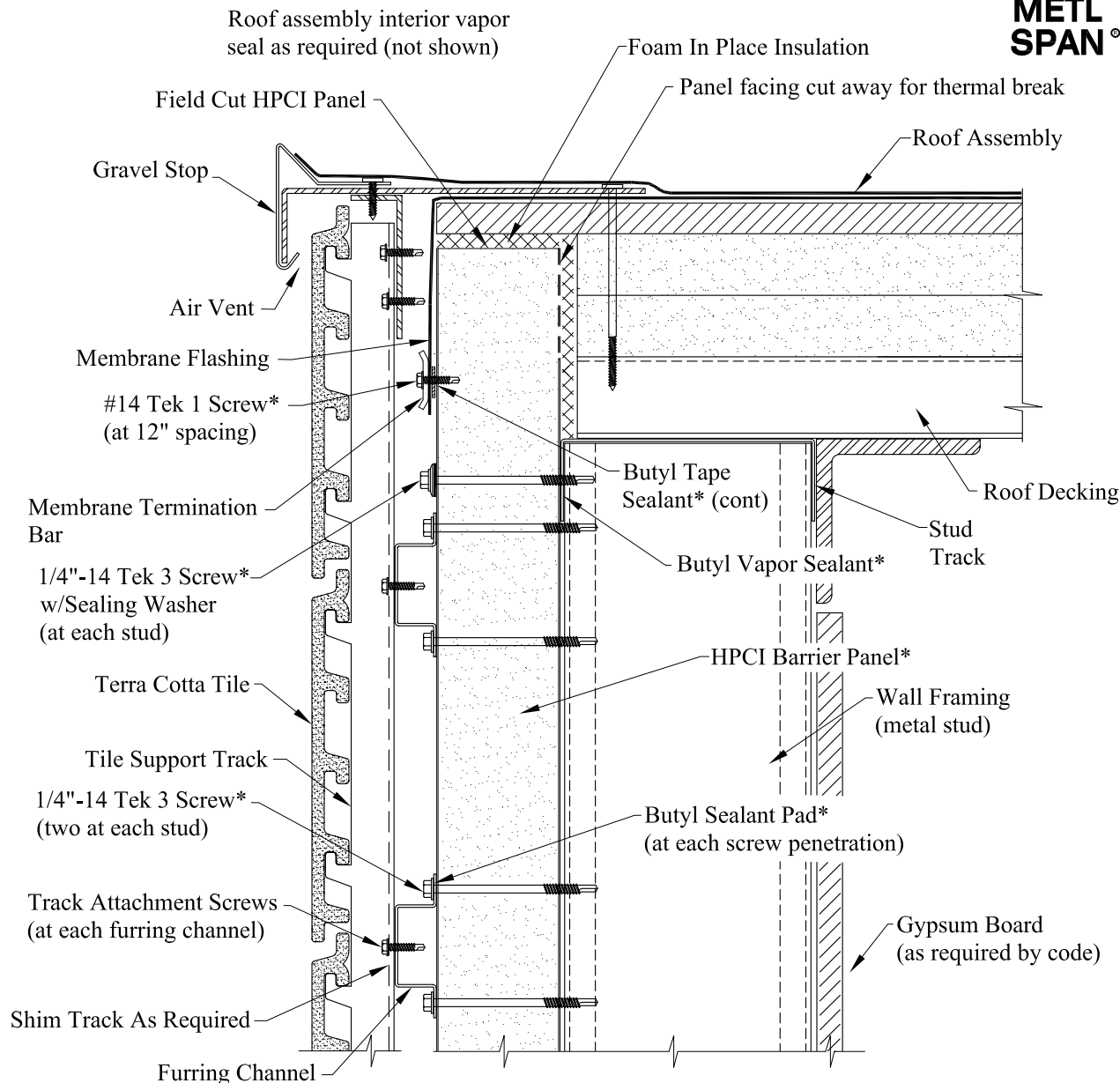
Wall Section @ Eave
