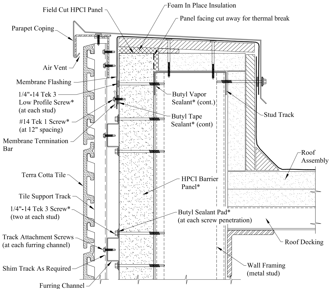
Wall Section At Parapet
