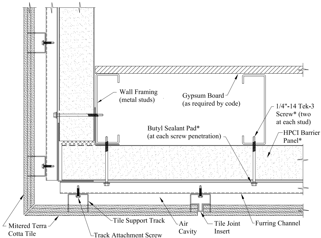
Wall Plan @ Outside Corner
