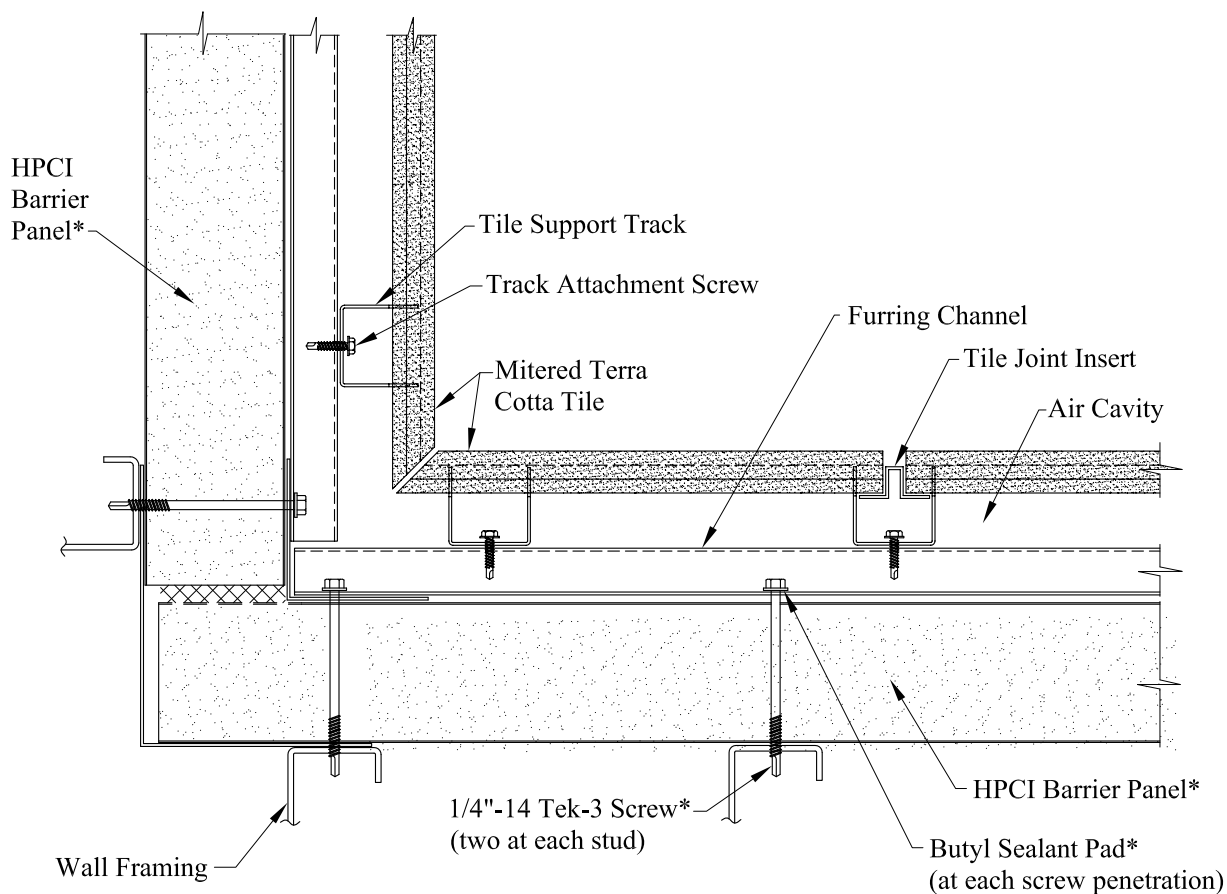
Wall Plan @ Inside Corner
