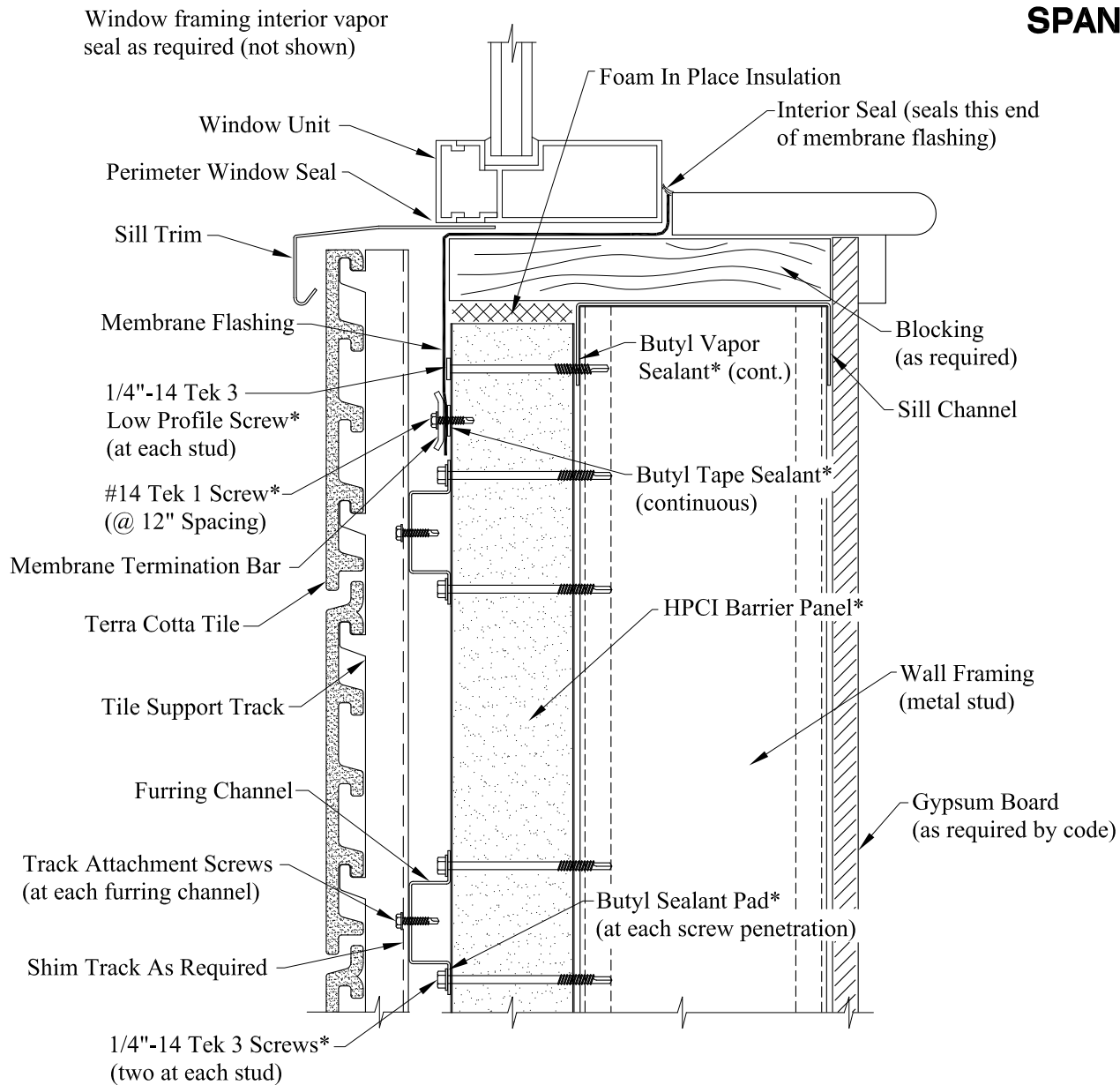
Wall Section @ Window Sill
