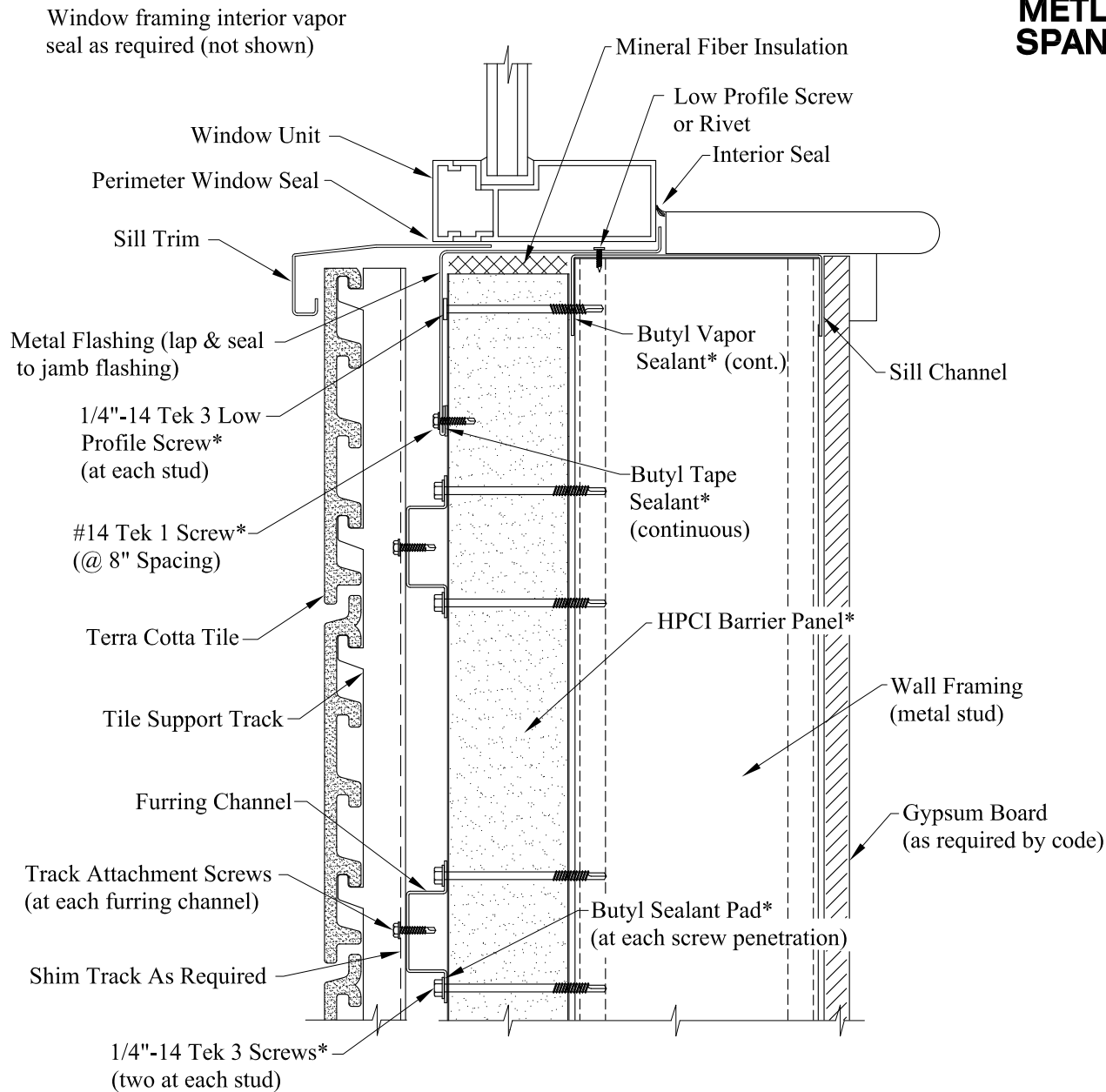
Wall Section @ Window Sill
