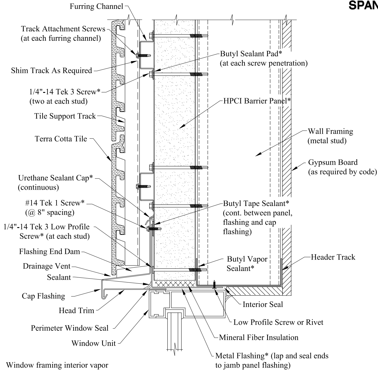
Wall Section @ Window Head
