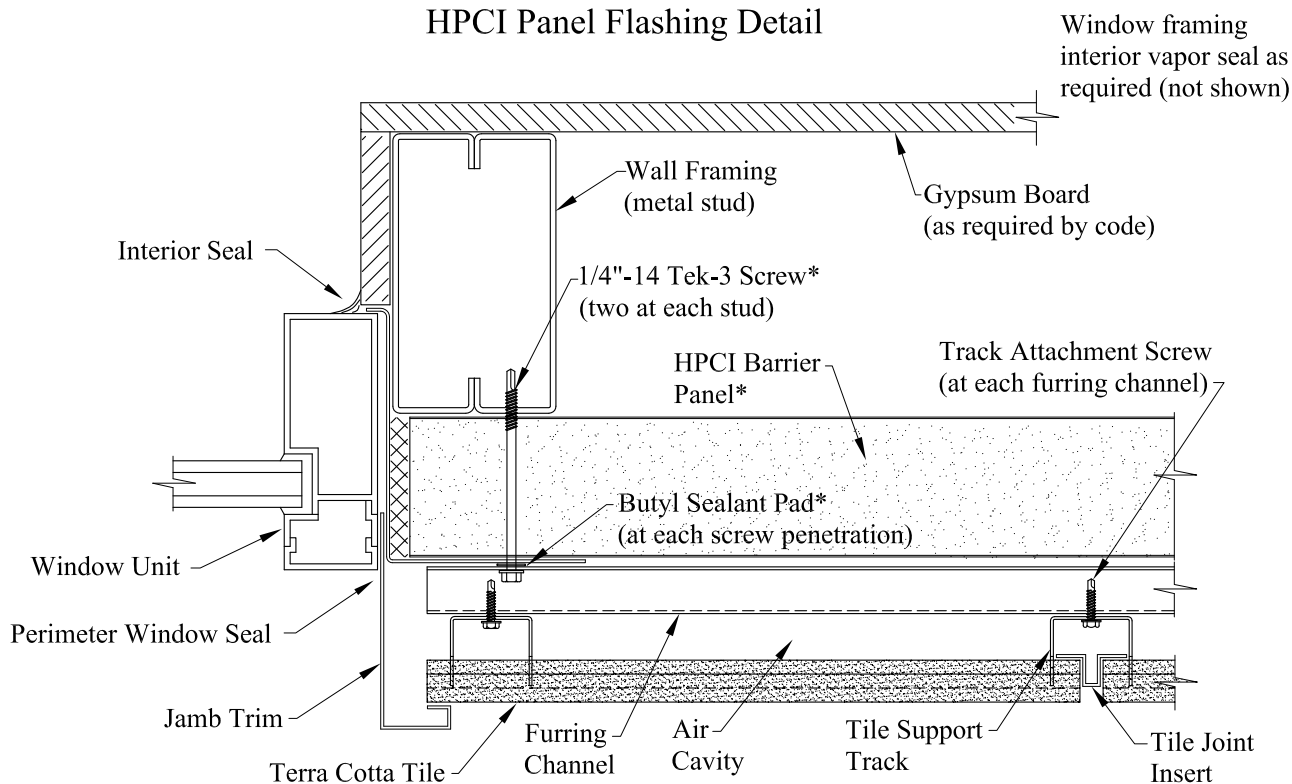
Wall Plan @ Window Jamb
