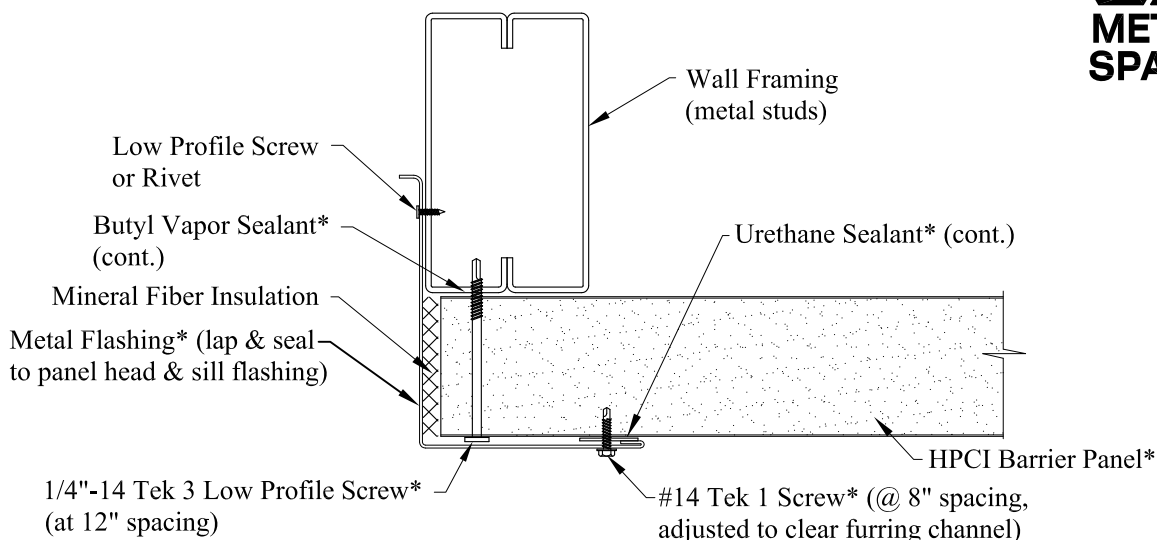
HPCI Panel Flashing Detail
