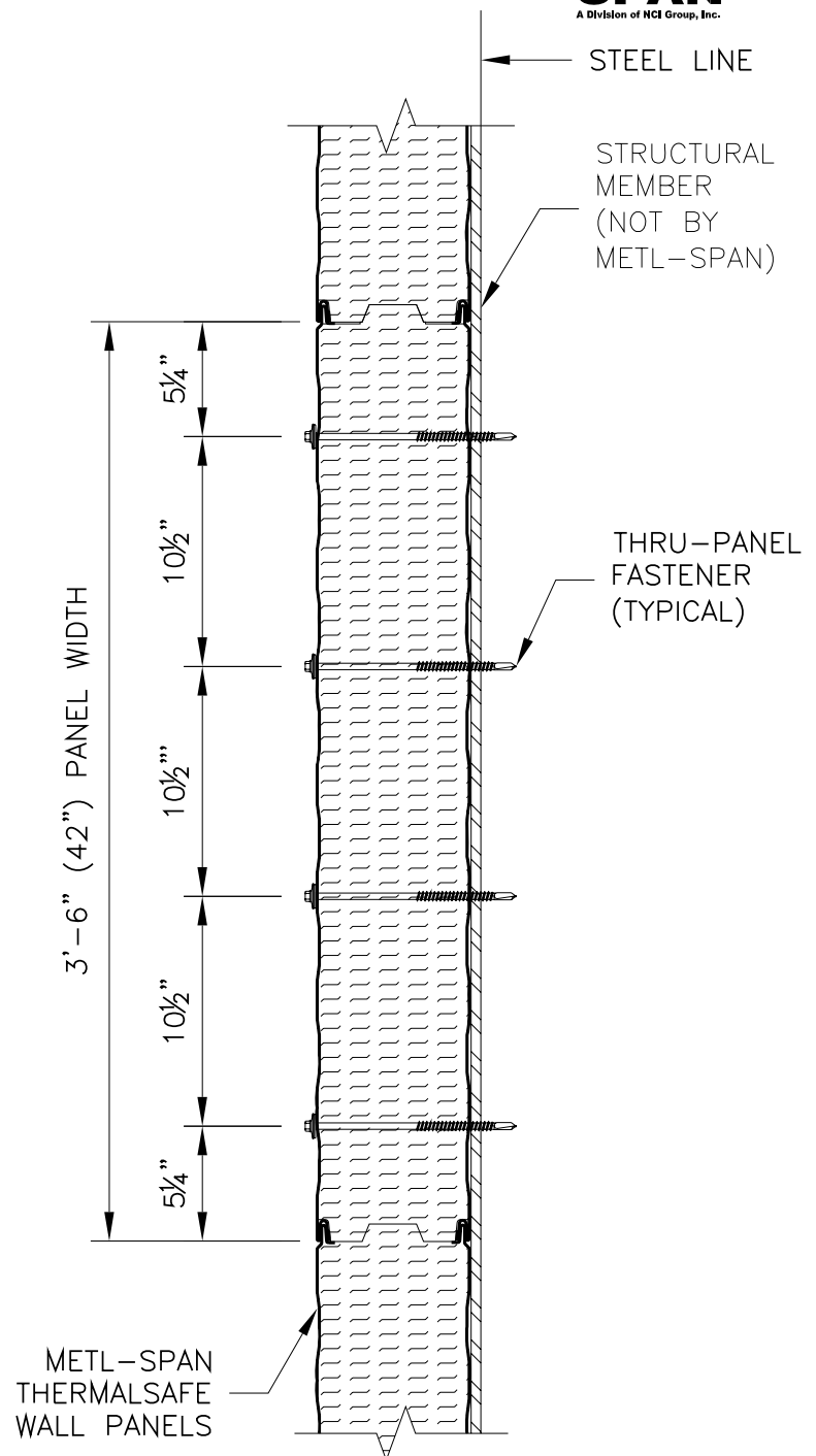
FASTENER PATTERN 2
