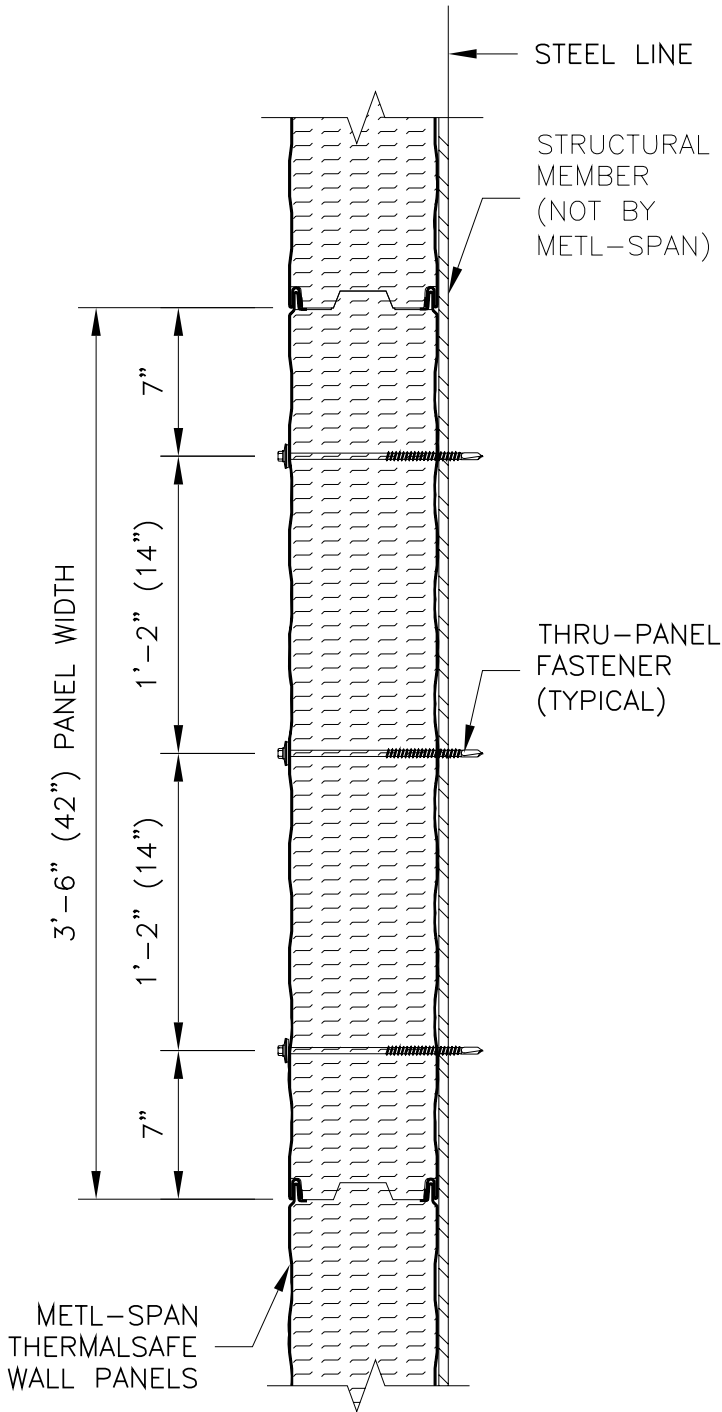
FASTENER PATTERN 1
