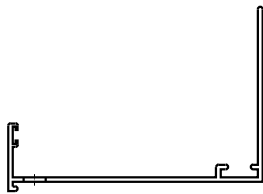
4" BASE EXTRUSION [9404A]
