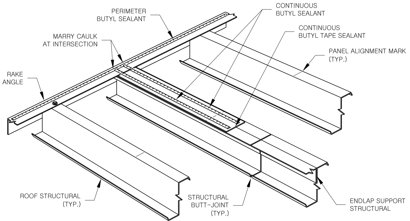
ENDLAP SUPPORT STRUCTURAL SECTION
