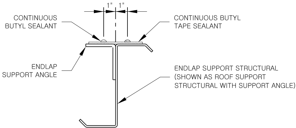
ENDLAP SUPPORT STRUCTURAL SECTION
