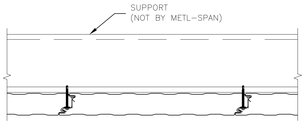
(FP1) SIDE JOINT CLIP ONLY
