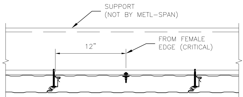
(FP2) SIDE JOINT AND (1) BLIND RIVET
