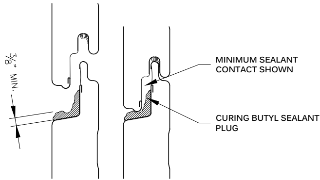
SEALANT PLUG DETAIL APPLY SEALANT AS PANELS ARE ERECTED
