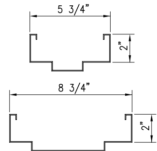
Frame Sections
