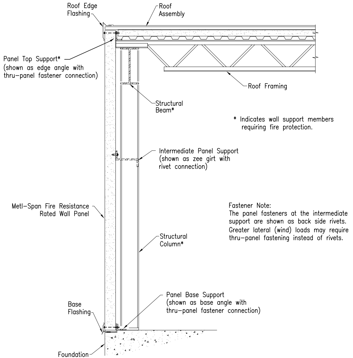
Typical Exterior Wall Section
