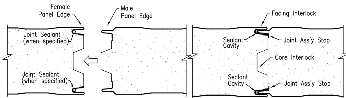
PANEL EDGES BEFORE ASSEMBLY
