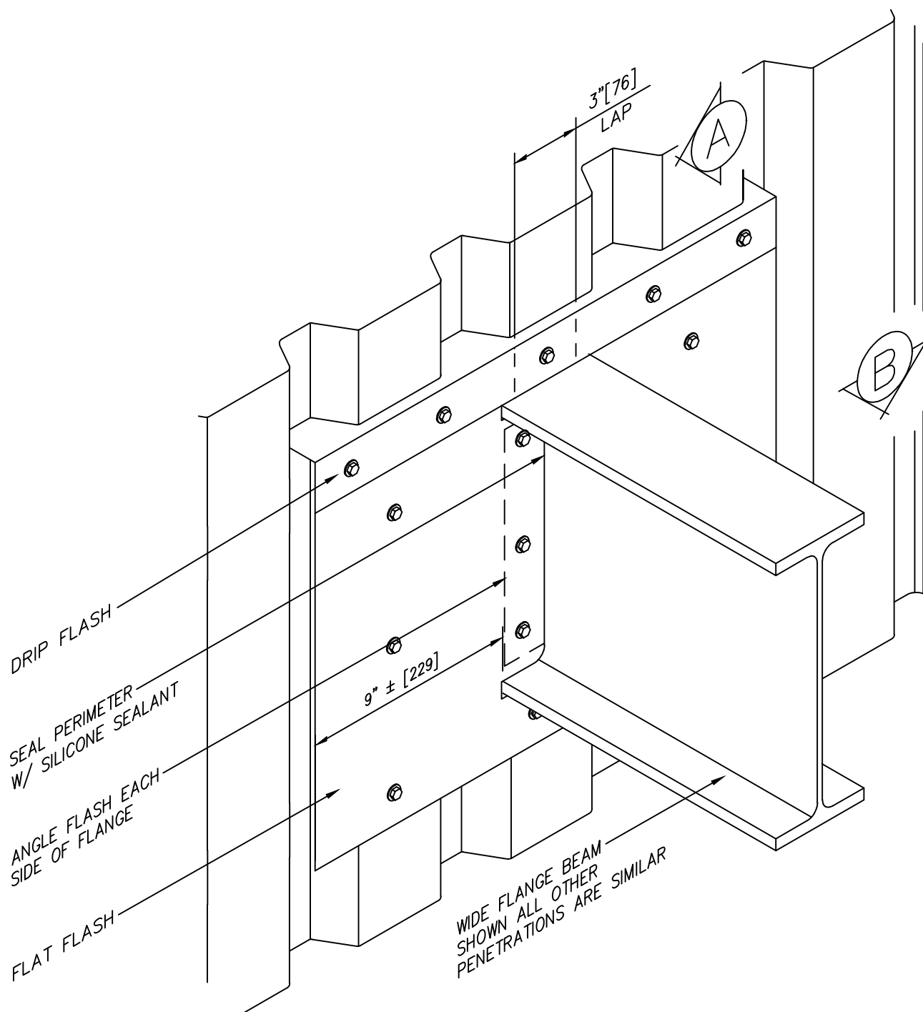
DETAIL 15 PENETRATION
