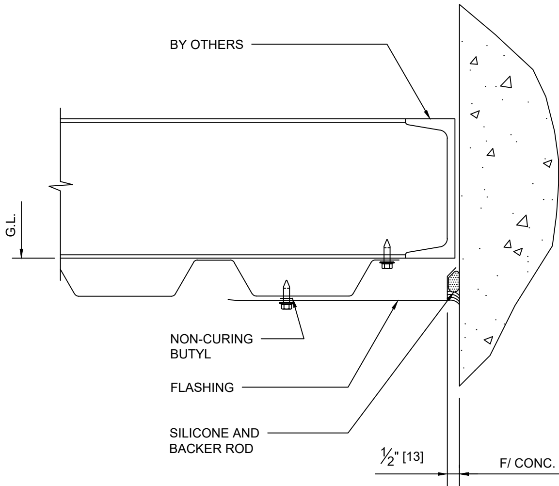
DETAIL 11 ENDWALL
