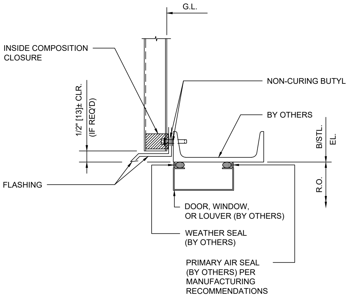
DETAIL 4 HEAD OPENING
