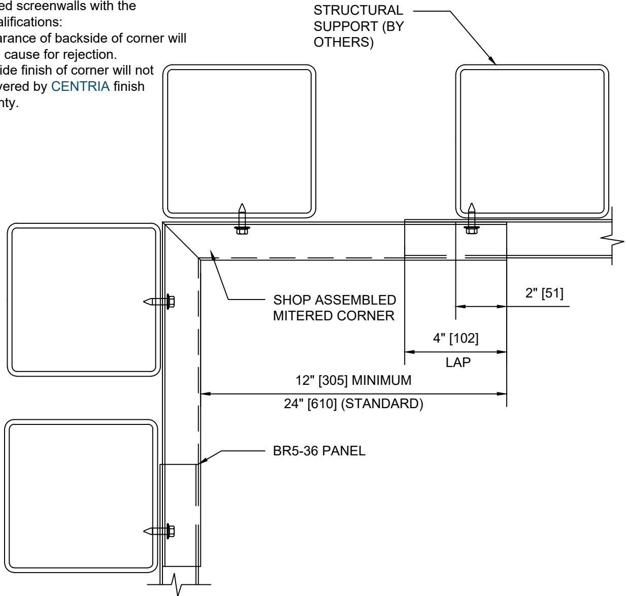
DETAIL 10A INSIDE MITERED CORNER - SCREEN WALL
