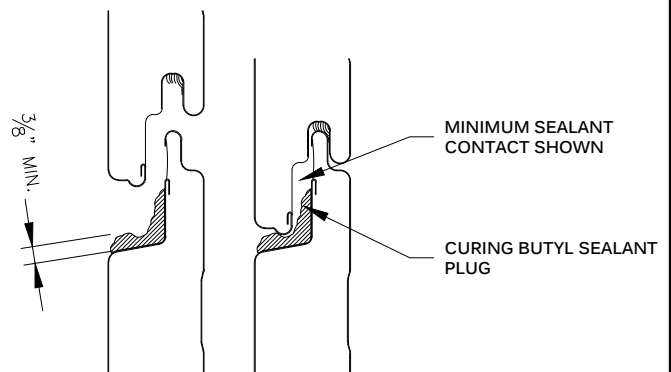
SEALANT PLUG DETAIL
