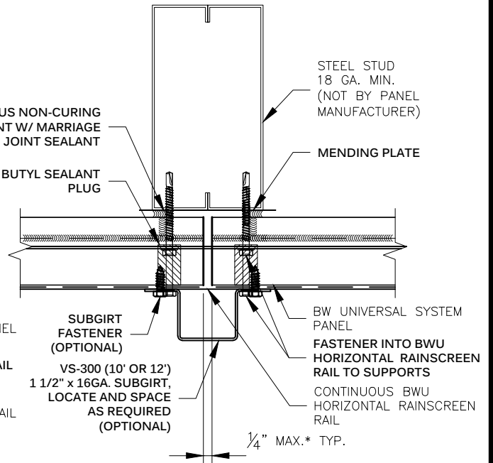
VERTICAL JOINT @ DOUBLE STUD
