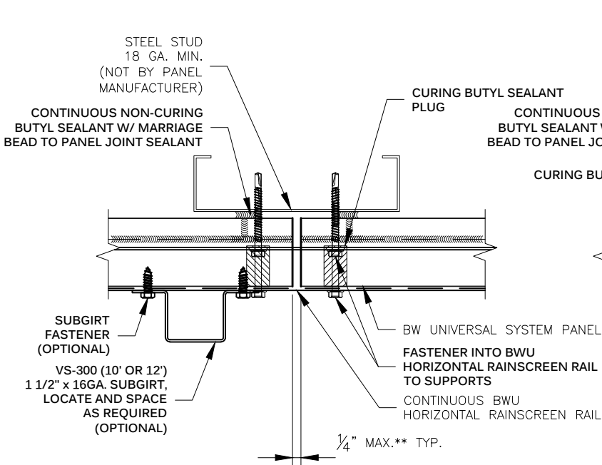
VERTICAL JOINT NOT @ **STUD
