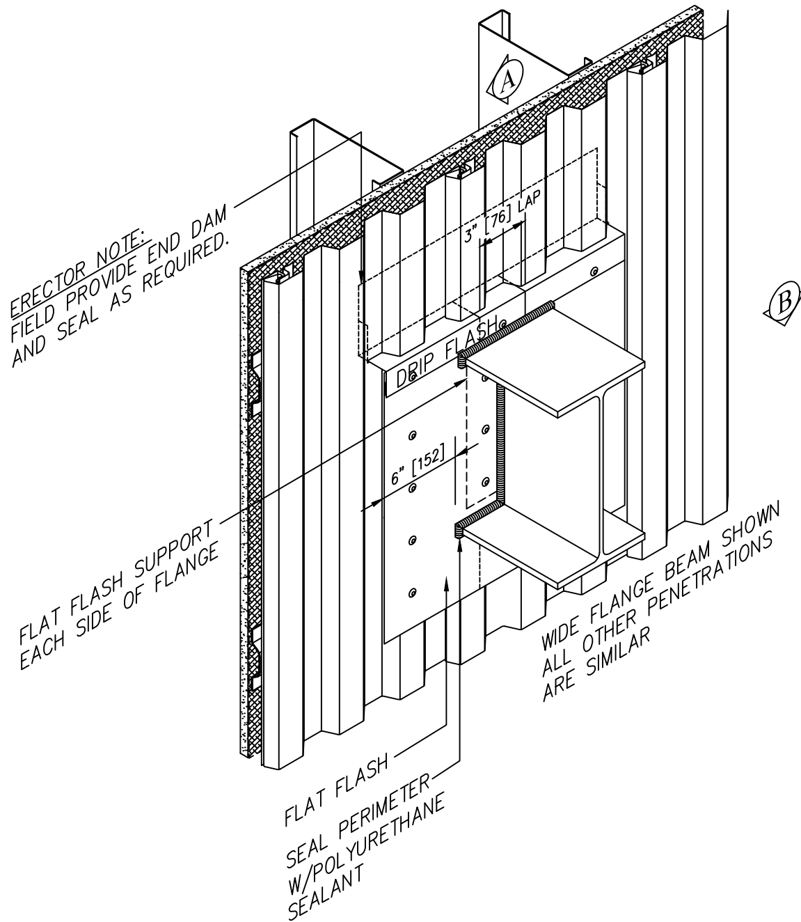
DETAIL 15 PENETRATION
