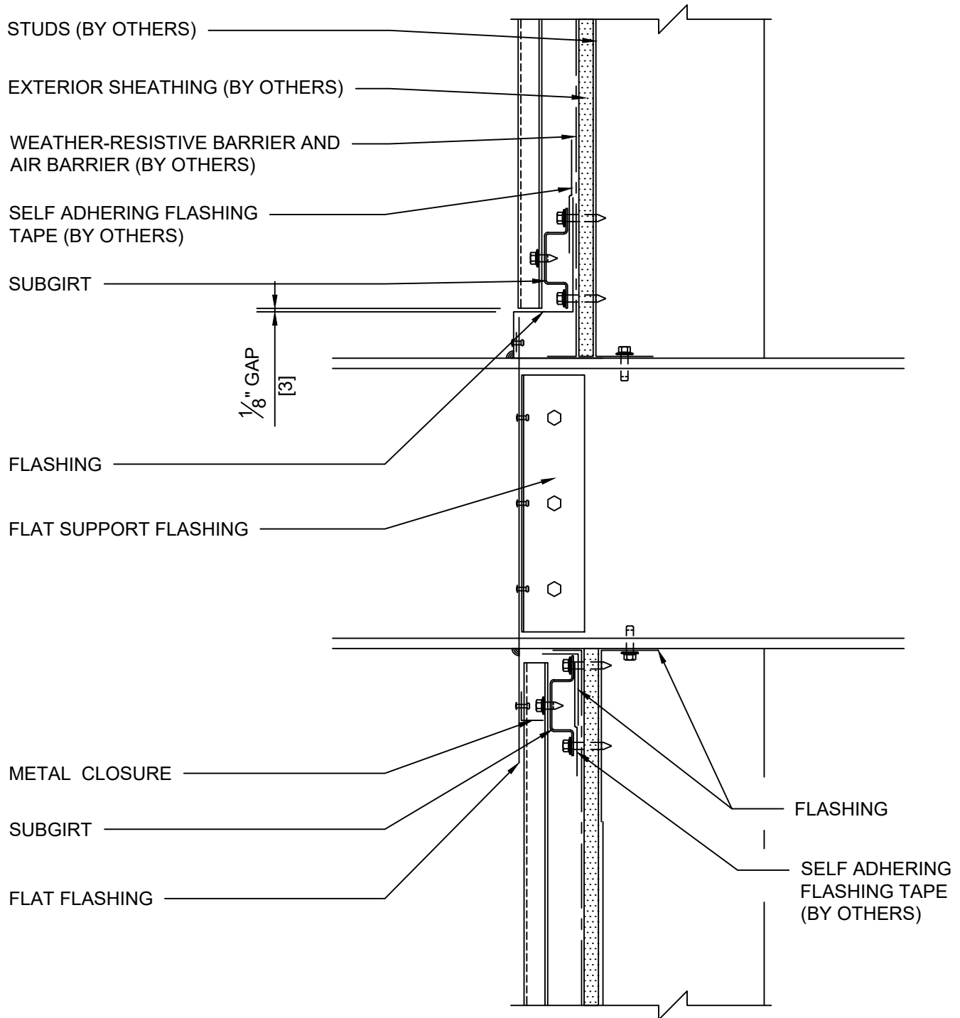
DETAIL 15A PENETRATION (SECTION A-A)
