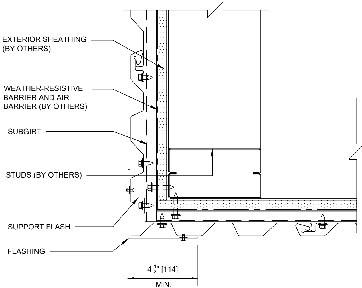
DETAIL 9 OUTSIDE CORNER
